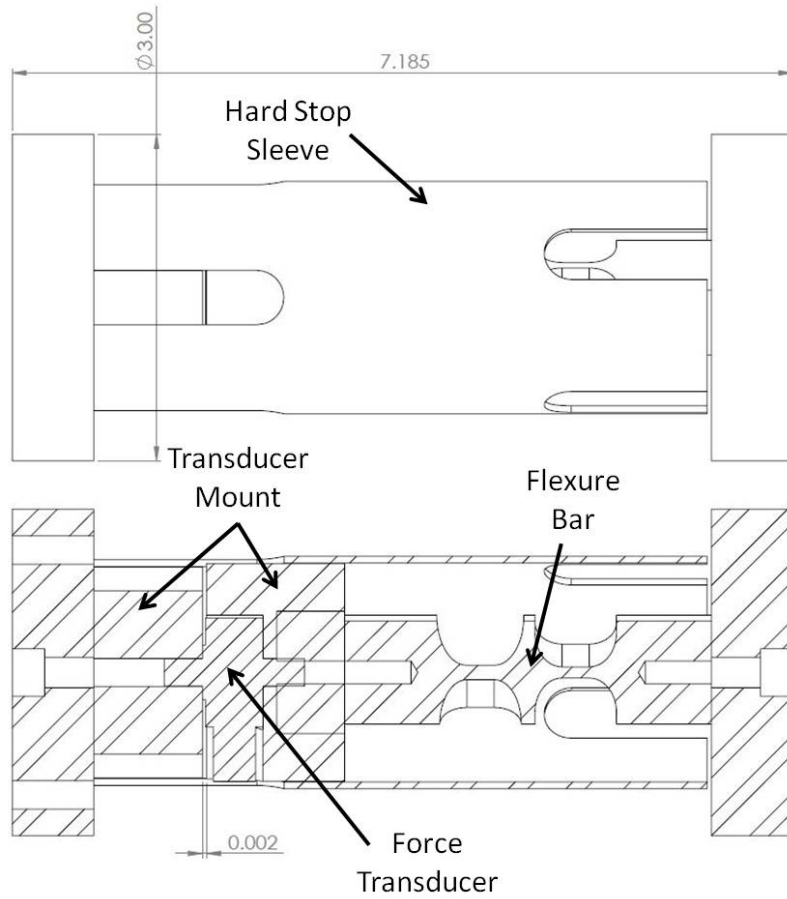
Figure 5.8: New transducer mount design
