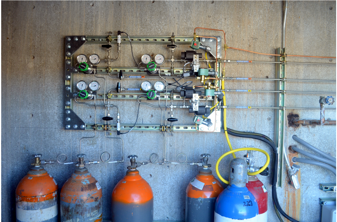
Figure 4.6: Installed Nitrogen Supply Panel
