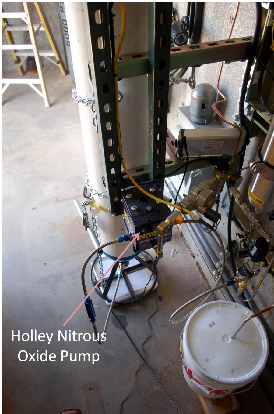
Figure 4.14: Holley nitrous oxide pump installed
