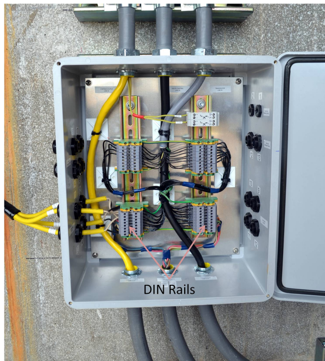
Figure 4.17: Fuel galley junction box
