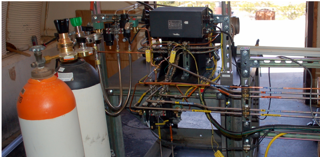
Figure 4.10: Rear view of rocket engine connections
