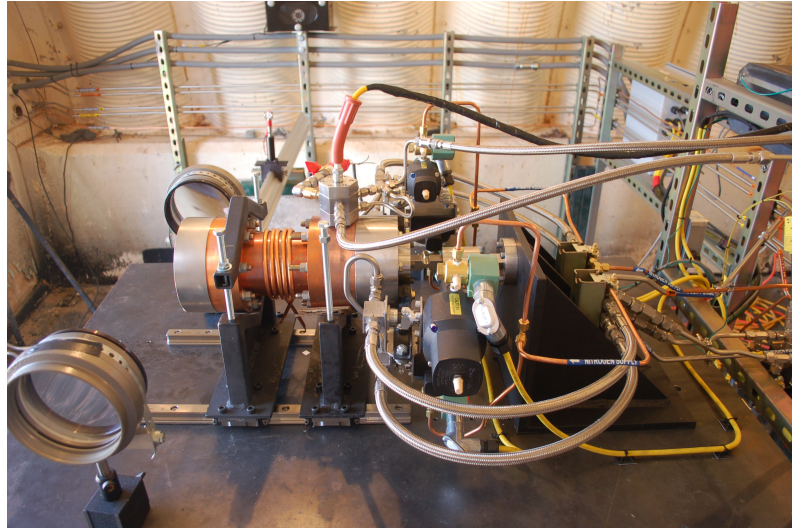
Figure 4.11: Side view of rocket engine connections
