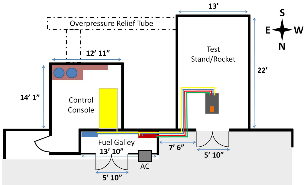
Figure 4.1: Final facility layout
